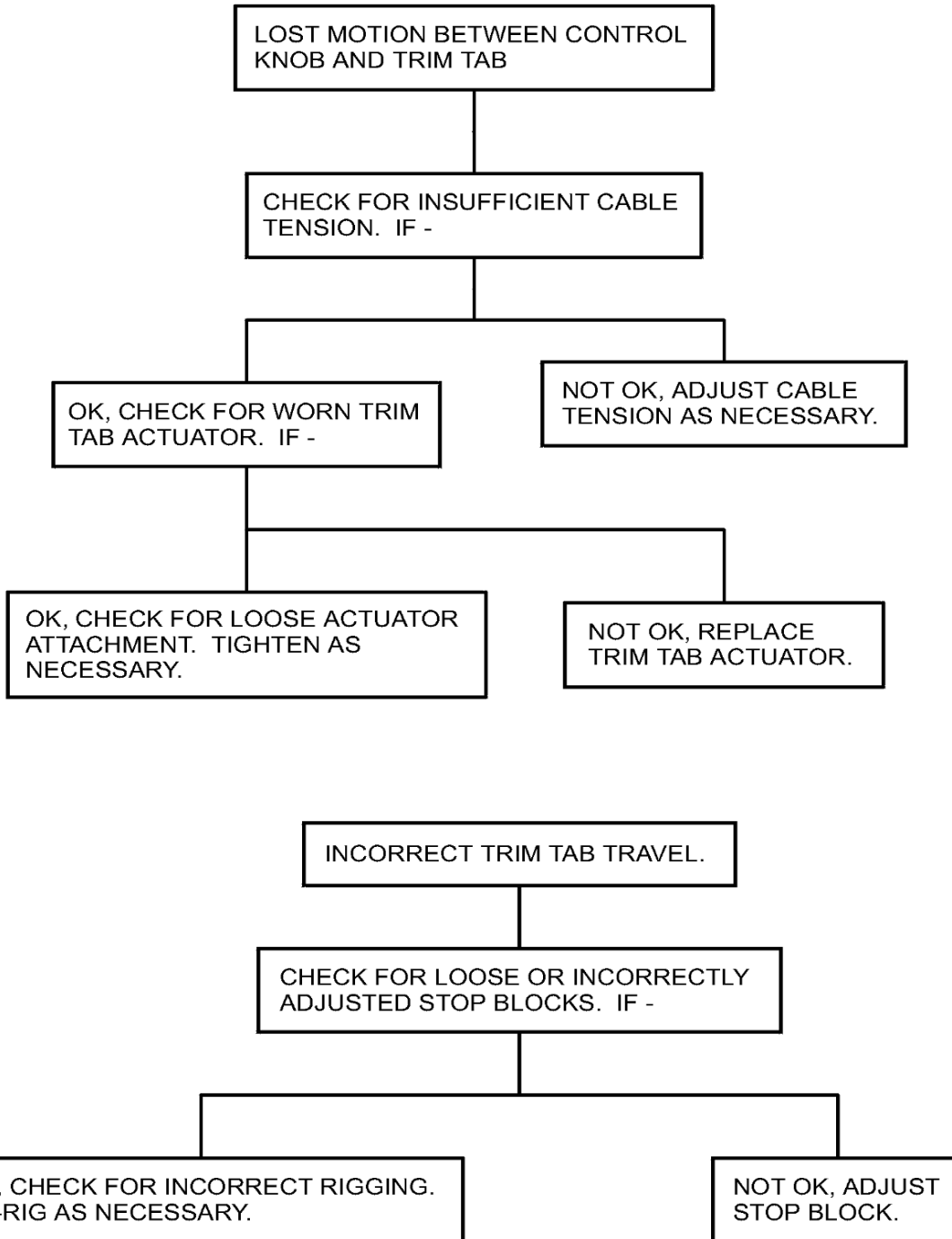
Figure 101 : Sheet 2 : Aileron Trim System Troubleshooting Chart
