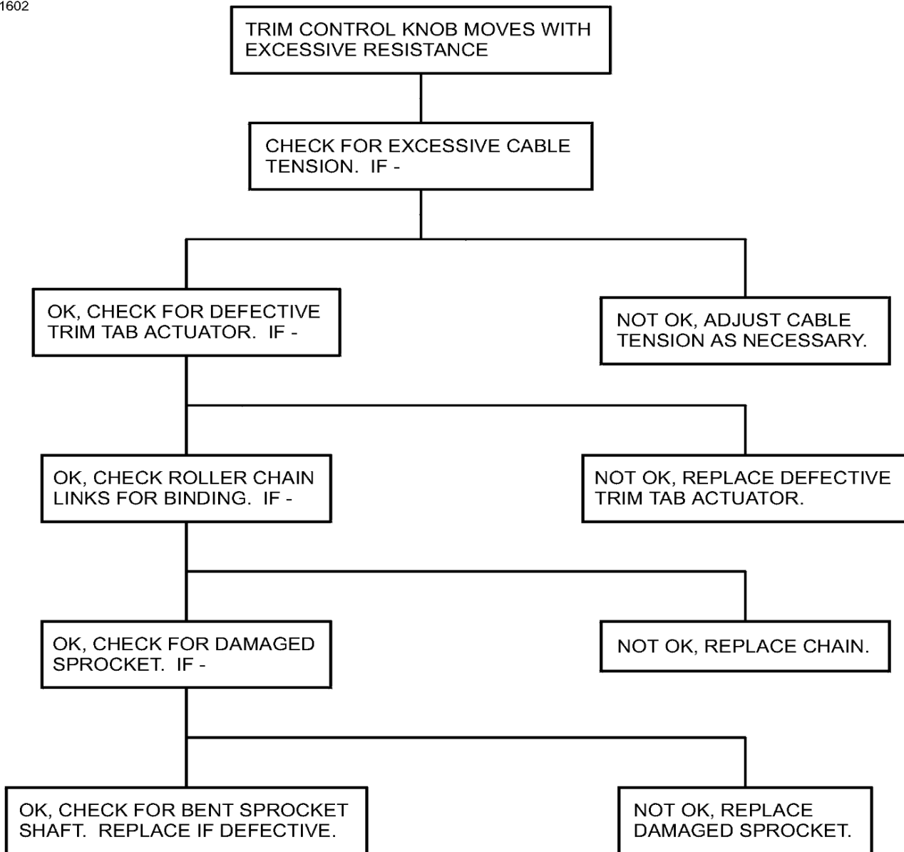
Figure 101 : Sheet 1 : Aileron Trim System Troubleshooting Chart
